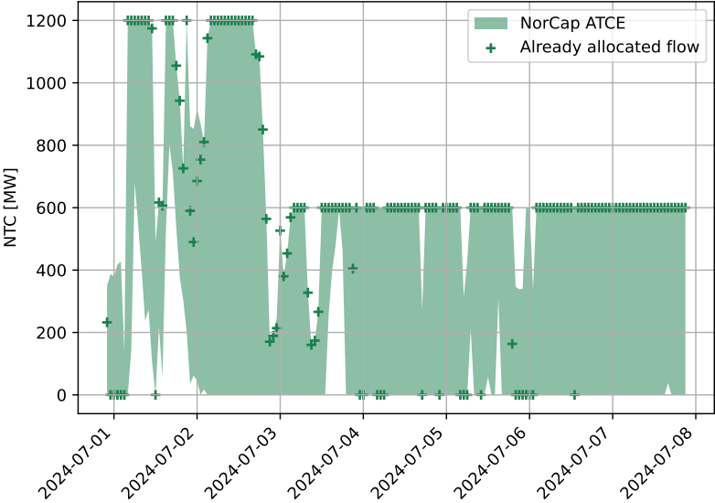
NTC SE3_SWL-SE4_SWL
