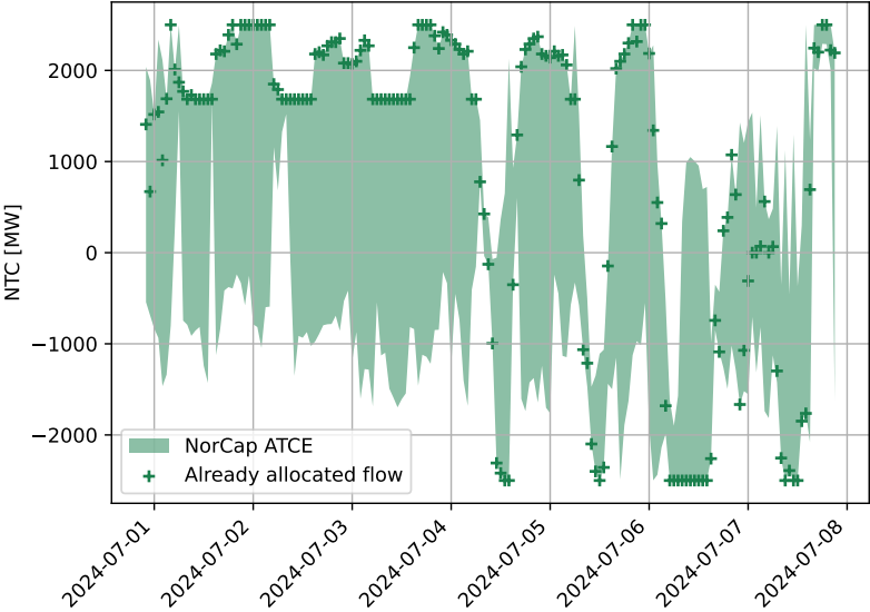
NTC DK1-DE_LU
